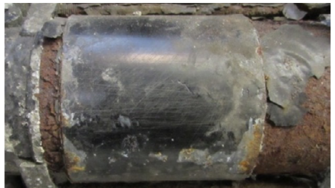
Heavy corrosion(Not off-vehicle condition)
