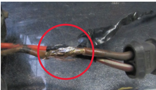
Cables shorter than 2 cm. Cables / wires damaged closer than 2 cm from housing.
